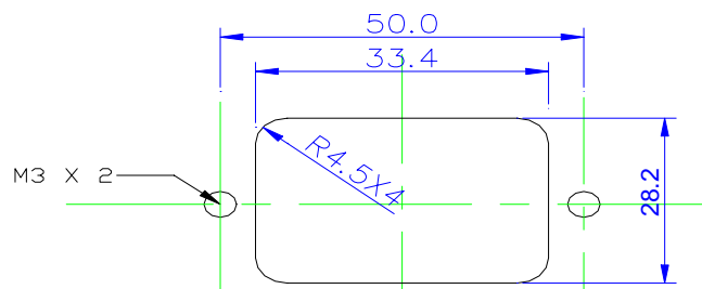
Panel Cut-out Size for FI-33 (for Front mounting Use)
